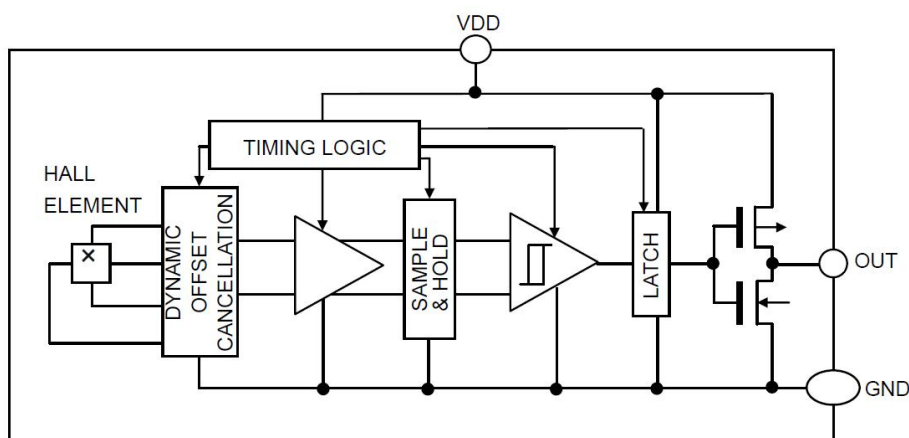
Figure 3, Block Diagram of AS1813
