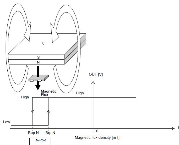
Fig 4, Magnetic Operation Characteristic of AS1813
