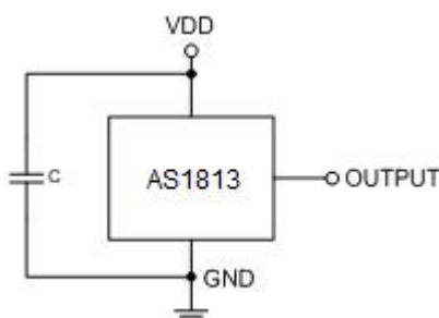
Figure 1, Typical Application Circuit of AS1813
